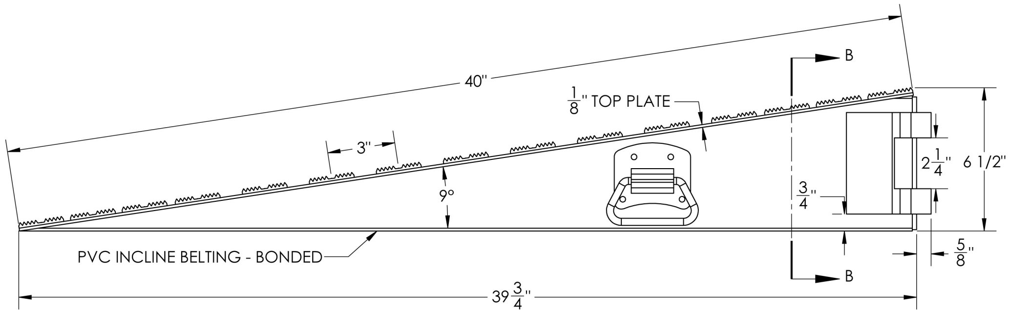
SECTION B-B
